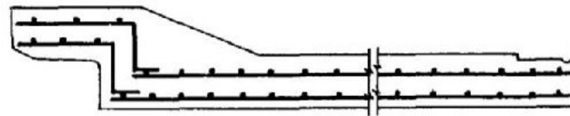
4B Socket Cage Longitudinal Suitably Bent for Connecting to Barrel Cage
