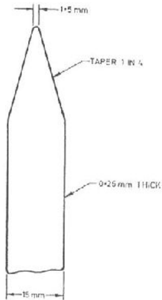
FIG. 2 GAUGE LEAP FOR MEASURING CRACKS
