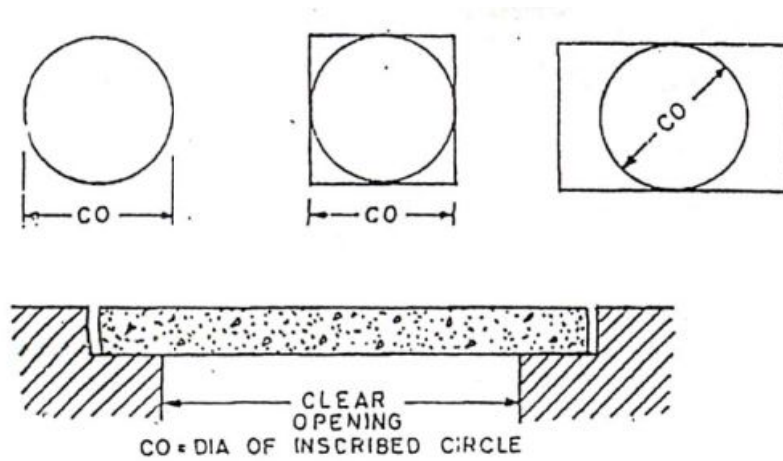
Fig.3 Illustration of Largest Incribed Circle in Clear Area
