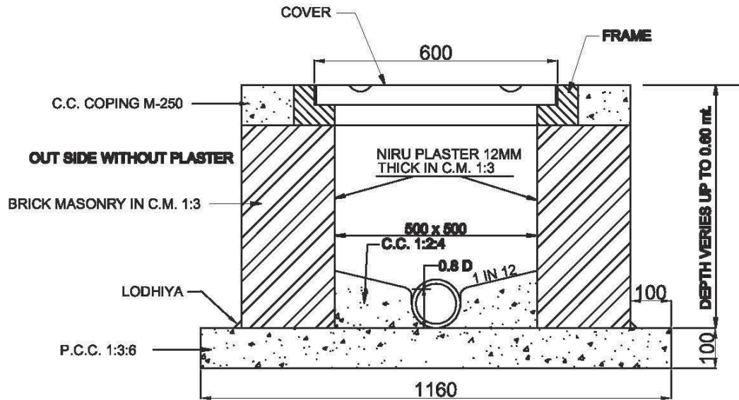
SECTIONAL ELEVATION
