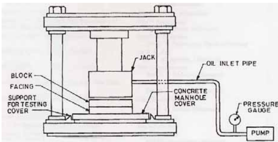
Fig.2 Arrangement For Load Test of Manhole Cover
