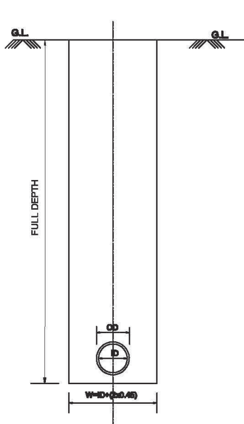
TRENCH CUT IN NORMAL CONDITION
