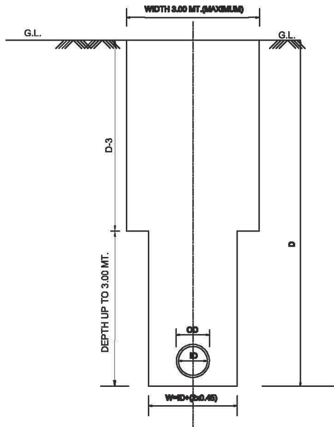
TRENCH CUT IN SPECIFIC CONDITION
